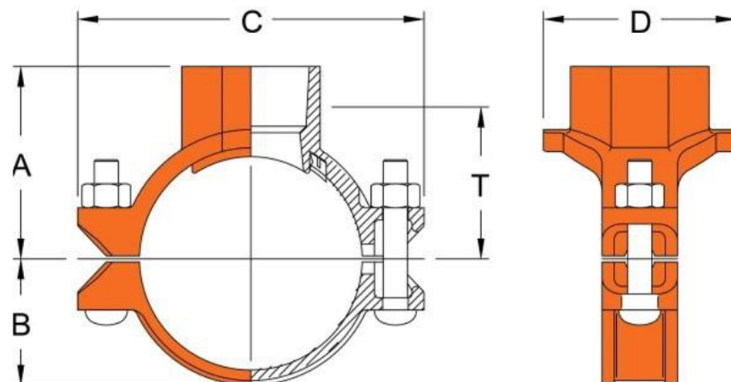
Model 7721 Mechanical Tee, Female Threaded Outlet
